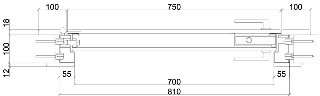
Cross section
